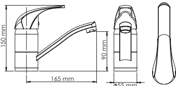
MEW single lever short spout sink mixer
