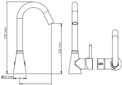
MES-G single lever gooseneck sink mixer
